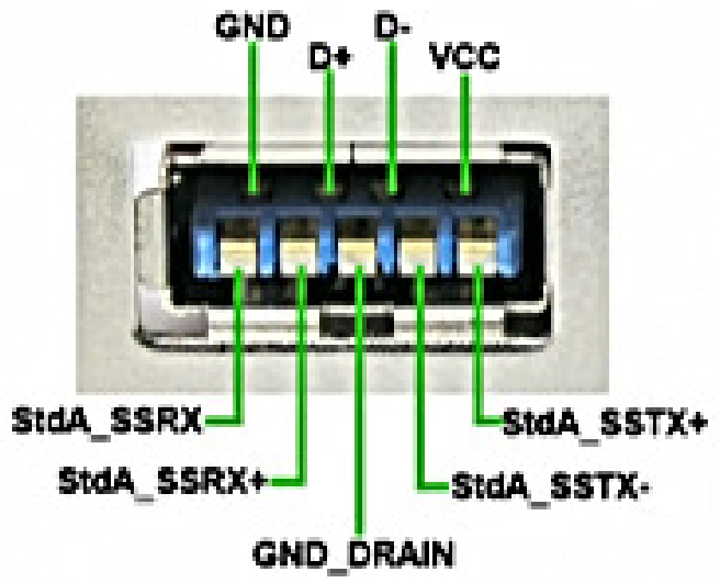
SuperSpeed standard A plug pinout
