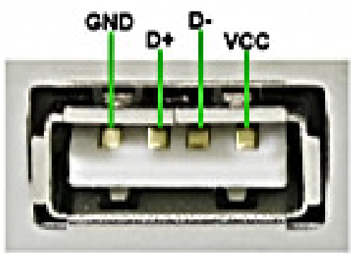
Hi-Speed USB 2.0 A plug pinout
