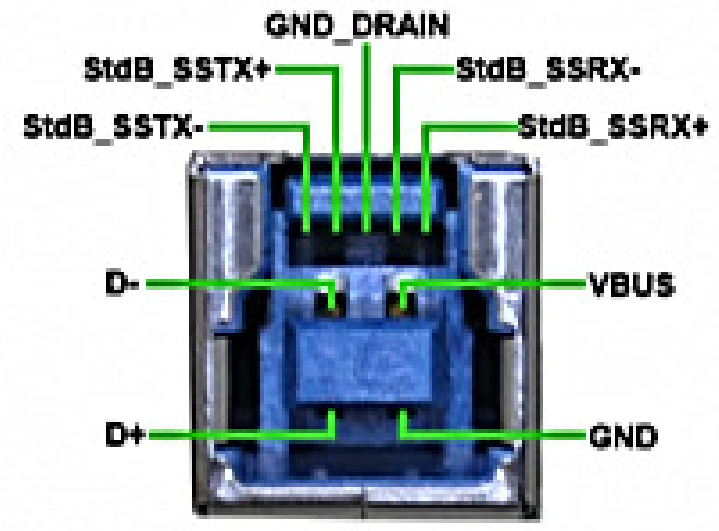
SuperSpeed standard B plug pinout
